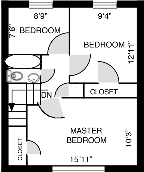
2ND LEVEL - 450 SQ. FT.
